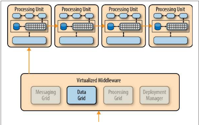
Figure 5-4. Data-grid component
